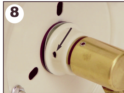
8 Align holes on reel axle with the holes in the bell cap.
